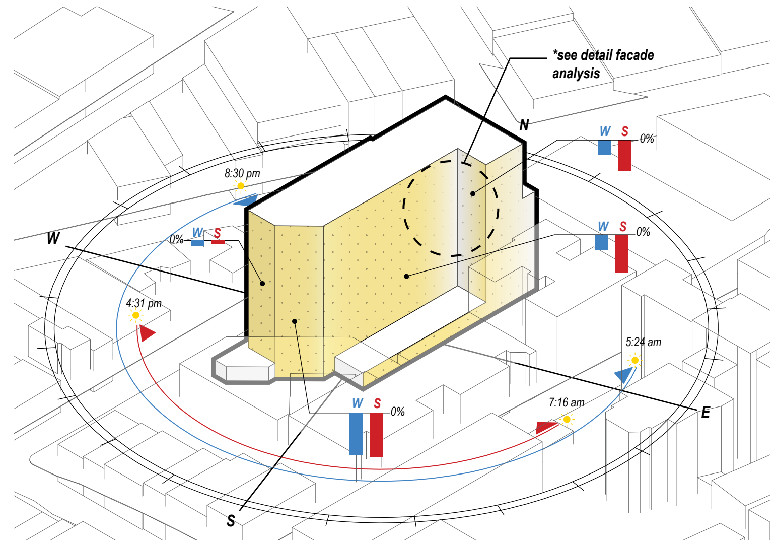
REAR AXON
